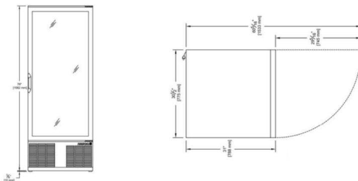
Front Elevation and Plan View (door swing)
